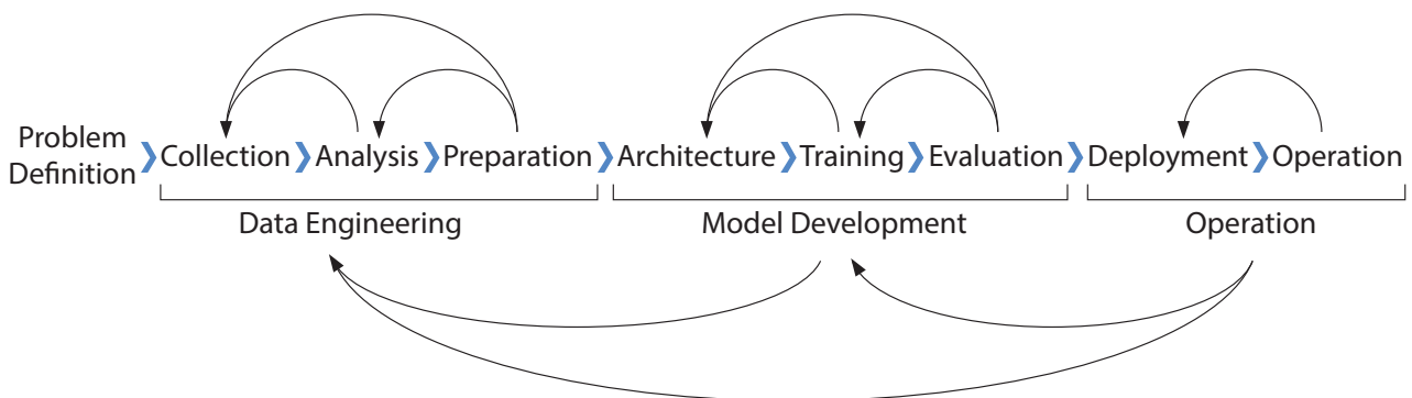
Figure 4.1. The life cycle of a classifier.
