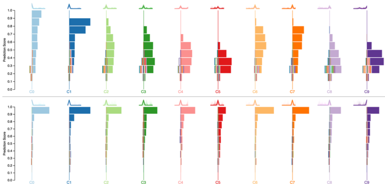
Figure 4.8. Squares [45] displaying the performance of two classifier (top: random forest, bottom: SVM) trained on the MNIST dataset. They yield the same accuracy of 0.87 , but show vastly different score distributions.
