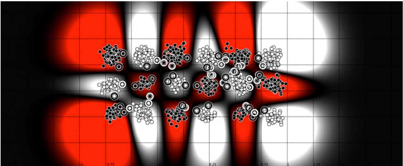
Figure 4.9. A visualization from MLDemos, showing the decision space of a binary SVM classifier using RBF kernel. White and red denotes different classes, and black represents uncertainty.
