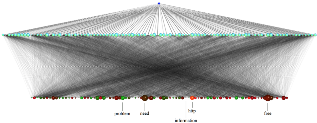
Figure 4.5. A spam classifier, where each input is a term in the email. The input data of the network is a subset of the spam in the training set [58].
