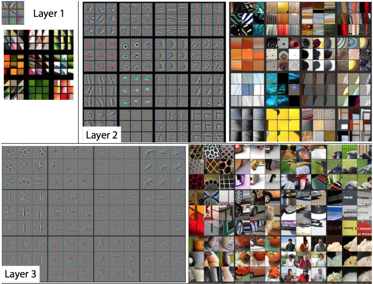
Figure 3.5. Visualization of a CNN generated using the de-convolution method [65]. Gray images in the left are the top nine activations in a random subset of neurons across validation data, projected back to image space. In the right are corresponding image patches.
