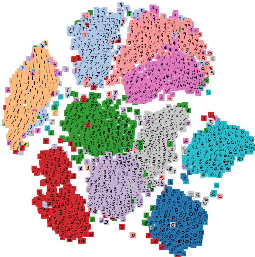
Figure 4.3. The t-SNE projection of the MNIST dataset, colored by the labeled digits.
