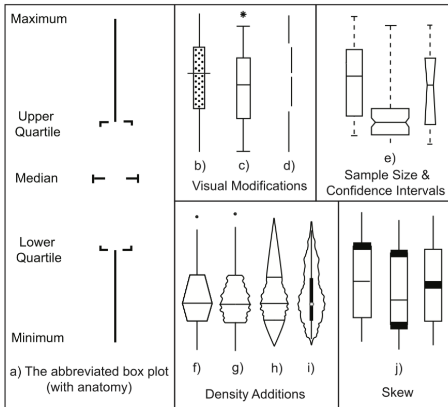
Figure 4.2. Variations on the box plot [41]. a) Abbreviated box plot. b) Range plot. c) Box plot. d) Interquartile plot. e) Variable width and notched box plots expressing sample sizes and confidence levels. f) Hist plot. g) Vase plot. h) Box-percentile plot. i) Violin plot. j) Skew and modality plots.
