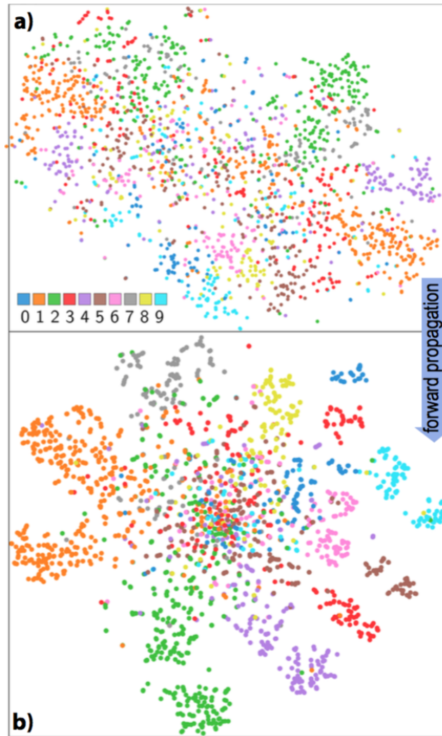
Figure 4.4. Projection of the MLP hidden layer activations after training [44], SVHN test subset. a) First hidden layer. b) Last hidden layer.
