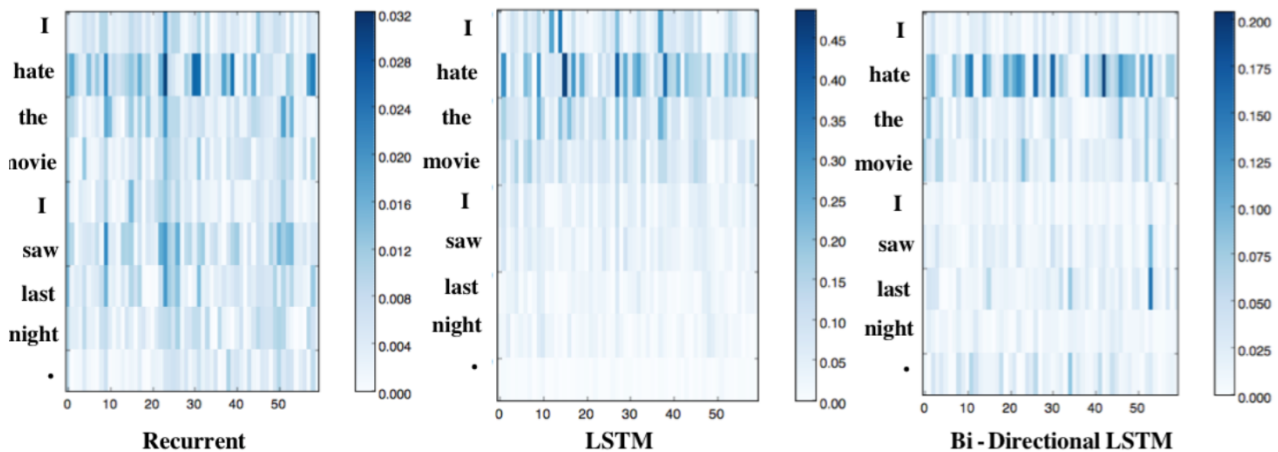
Figure 3.4. Saliency matrix maps for “I hate the movie I saw last night.” of three RNN sentiment classifiers. Left : a vanilla RNN; Middle : an LSTM; Right : a bi-directional LSTM [50].
