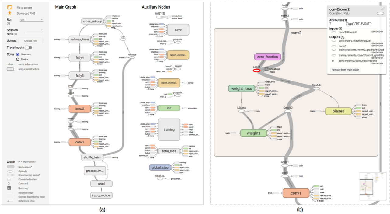
Figure 4.7. The TensorFlow Graph Visualizer shows a CNN image classifier [63]. (a) An overview displays a dataflow between groups of operations, with auxiliary nodes extracted to the side. (b) Expanding a group shows its nested structure.
