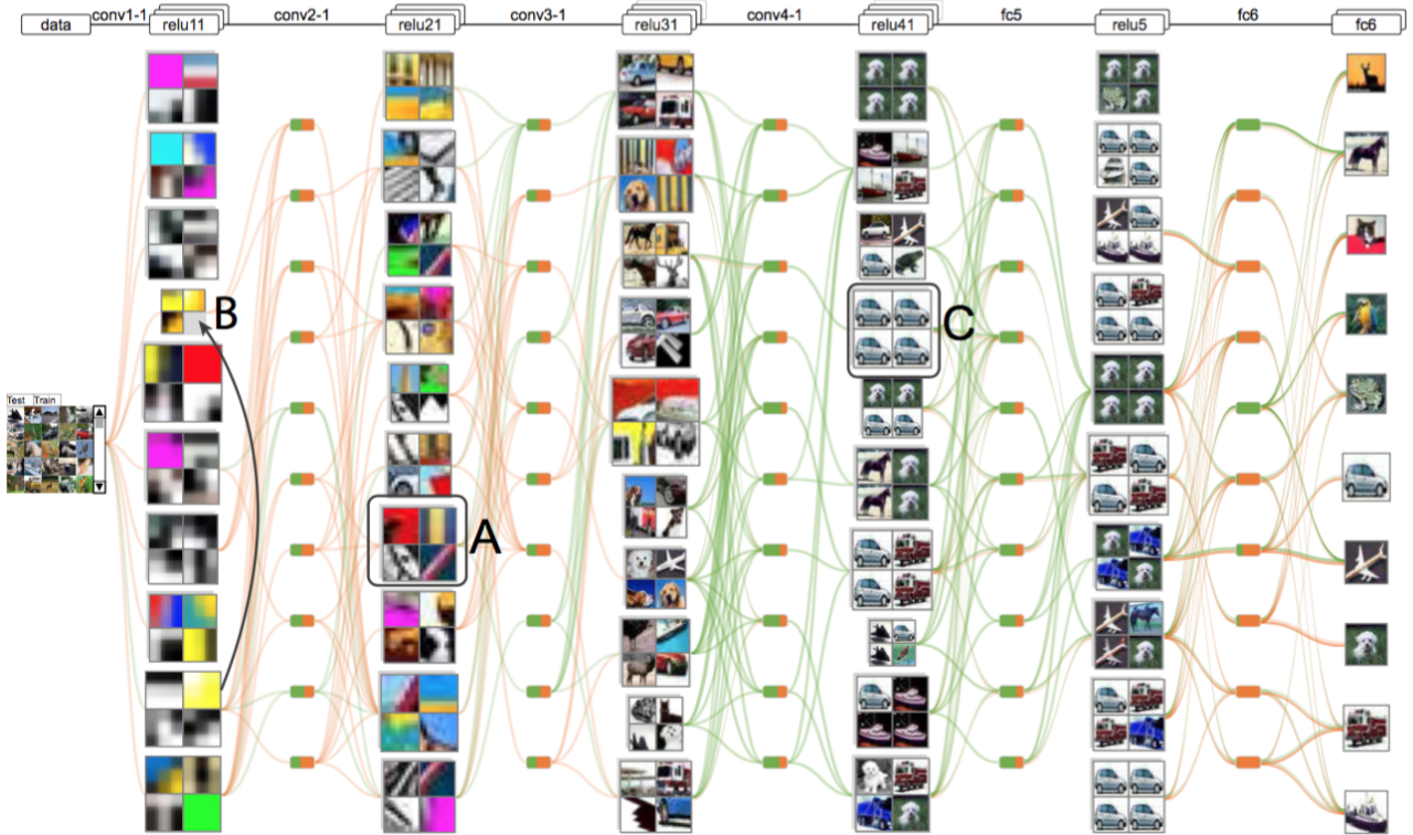
Figure 4.6. A visualization of a CNN with a large number of layers and neurons using neuron clustering and edge aggregation [32].
